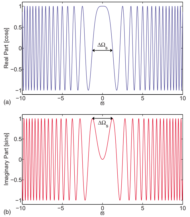
FIG. 2. (Color online) The real (top) and imaginary (bottom) parts of the exponential in Eq. (17). \phi is defined to be \phi = \beta_2 z (\omega - \Omega_S)^2 / 2 = a\varpi^2 , where a = \beta_2 z \Omega_S^2 / 2 and \varpi = \omega / \Omega_S - 1 , which is the normalized frequency. a = 1 is used for the figure. Both \cos \phi and \sin \phi oscillate rapidly as \varpi varies from the origin. Only the frequencies in the central region of the two plots contribute to the temporal waveform at a particular time instant. Contributions from all the other frequencies oscillate rapidly between positive and negative values and cancel out when integrated over all frequencies.
